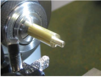
Turining down the cutter post
